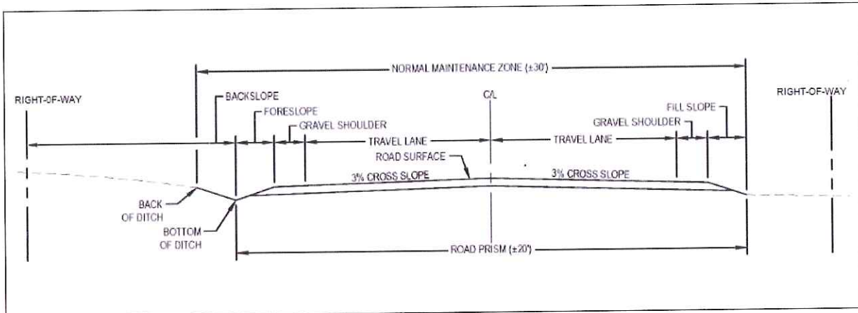
Figure 1. Typical Road Section for Gravel and Paved Surfaces
